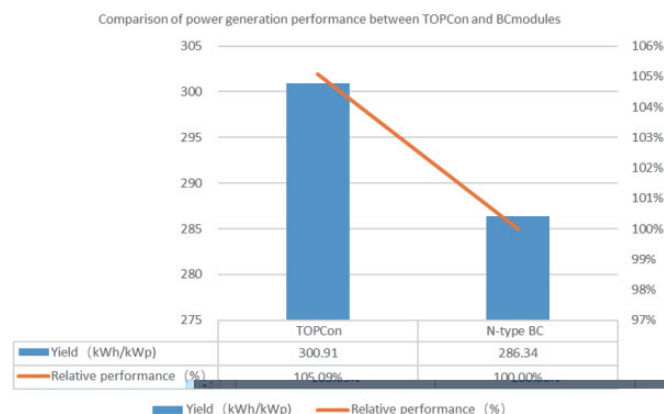
Figure 1: Comparison of power generation per watt between TOPCon and other BC II modules
